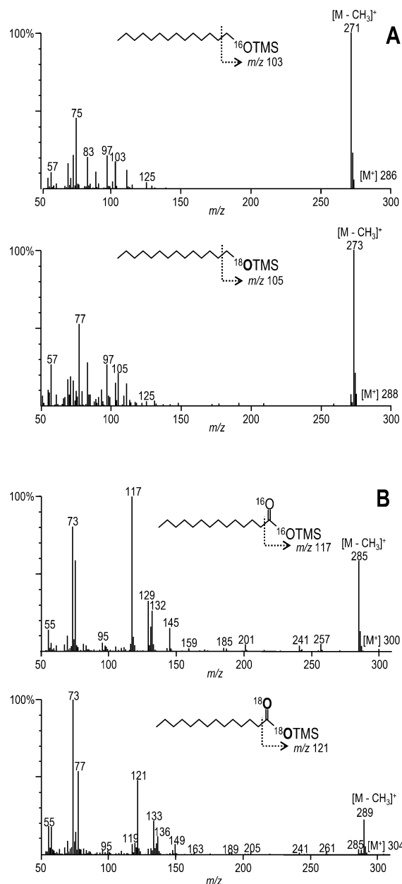
Figure 4. Mass spectra of 1-tetradecanol (A) and myristic acid (B) from Mro UPO reactions with n -tetradecane in ^{18}\text{O} -labeling experiments (bottom) and controls (top). The formulae for the unlabeled compounds found in the \text{H}_2^{16}\text{O}_2 reactions (A and B, top) and the labeled compounds found in the \text{H}_2^{18}\text{O}_2 (90 % isotopic purity) reactions (A and B, bottom) are shown as trimethylsilyl (TMS) derivatives.
